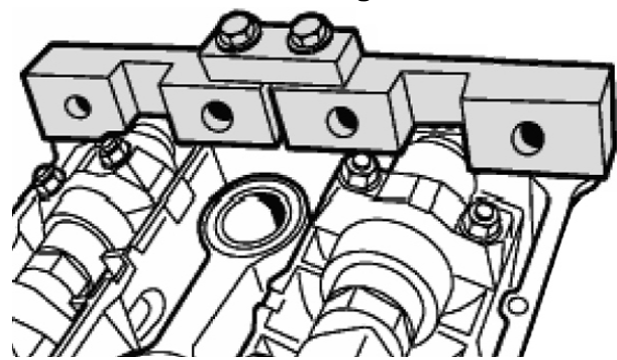
Camshaft Locking Tool
