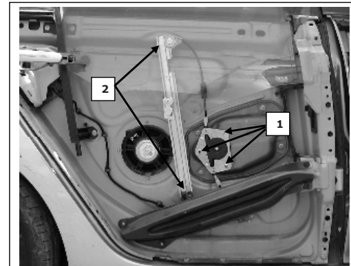
Porta lato destro, Portière arrière droite, Right rear door, Puerta lado derecho, Hinten rechte Tür, Porta traseira direita, Sag arka kapi, νόρτα οπίσθια δεξιά
