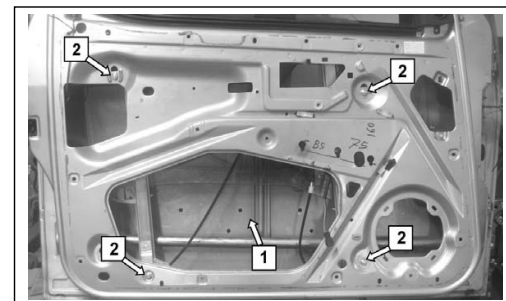
Porta lato destro, Portière avant droite, Right front door, Puerta lado derecho, Vorne rechte Tür, Porta frente direita, Sag on kapi, πόρτα εμπρός δεξιά
