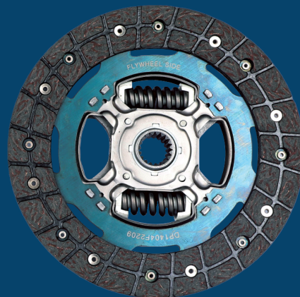
Aftermarket replacement driven plate
