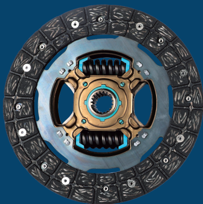
OEM driven plate with two torsional springs
