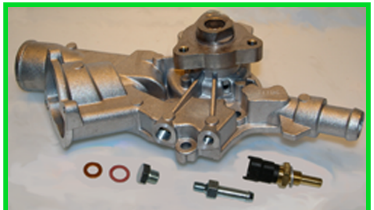
FWP 2194 - As FWP 2078 but with sensor unit and metal pipe
