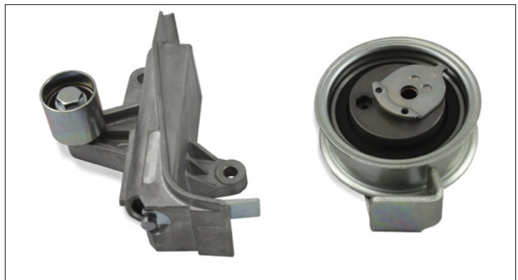
Fig. 1: Links trillingsdemper 533 0028 20, rechts spanrol 531 0531 20,
