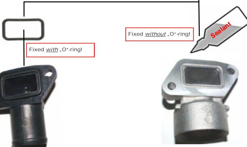
Plastic-connector
