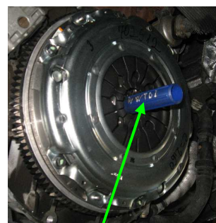
Centering tool
