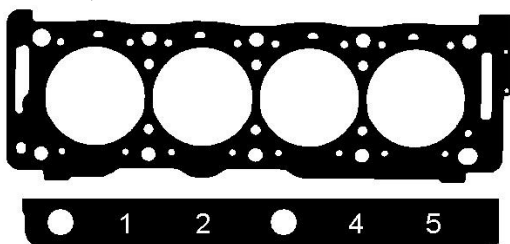
Elring 147.021
