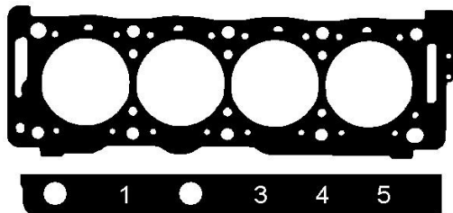
Elring 147.011
