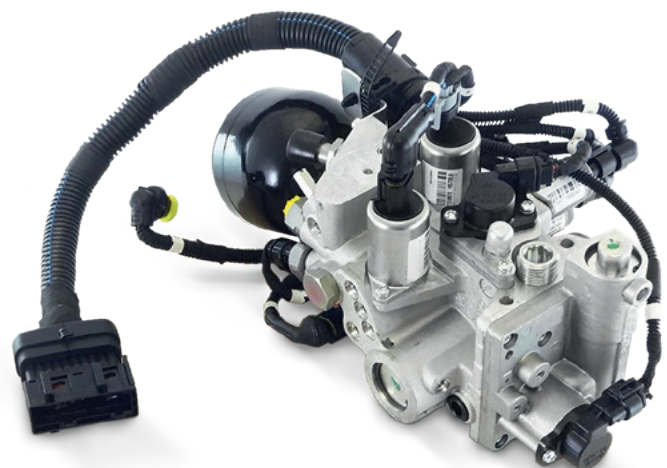
Selespeed manual gearbox (Alfa Romeo)
